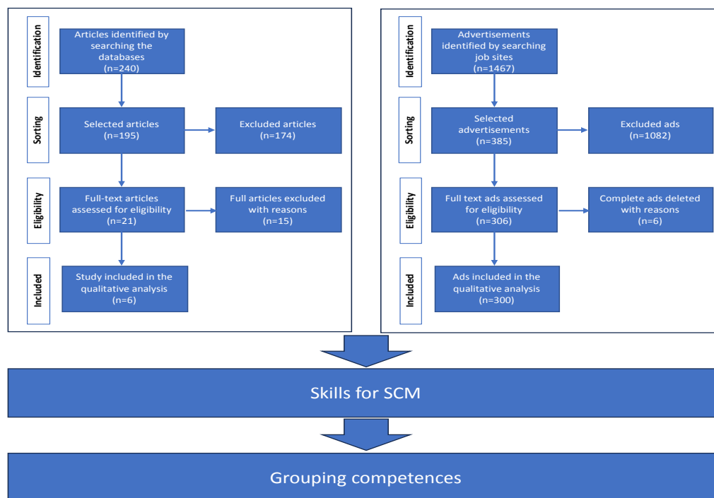
Fig. 6. Methodological approach
