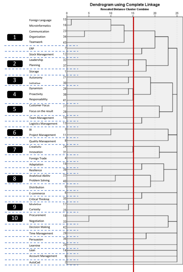
Fig. 5. Dendrogram grouping
